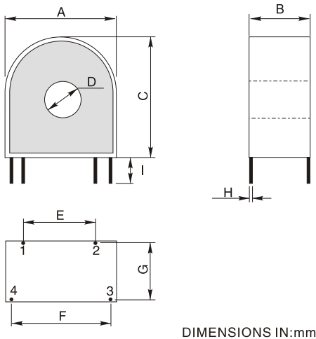
DIMENSIONS IN:mm
